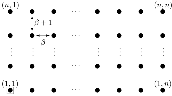
Fig. 3. Grid construction: n robots at (1,1) and m = n^3 targets on a (n \times n) rectangular grid; each of the n^2 gridpoints is a cluster of n targets. The intra-row distance is \beta , whereas the intra-column distance is \beta + 1 .
