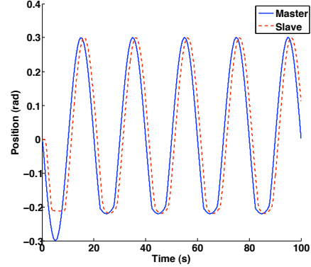
Fig. 7. Position tracking
