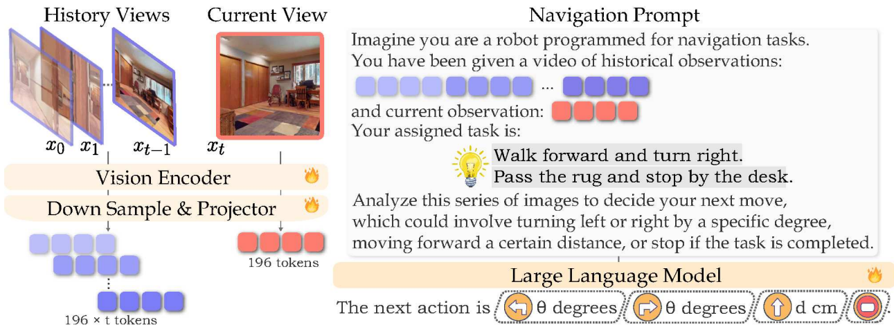
Fig. 3: Overview of our VLA framework. We denote the purple blocks (■) as memory tokens sampled from historical frames, and the red blocks (■) as the current observation tokens. 🔥 denotes trainable parameters. In our experiments, we tested configurations with 8 to 64 frames for t .
