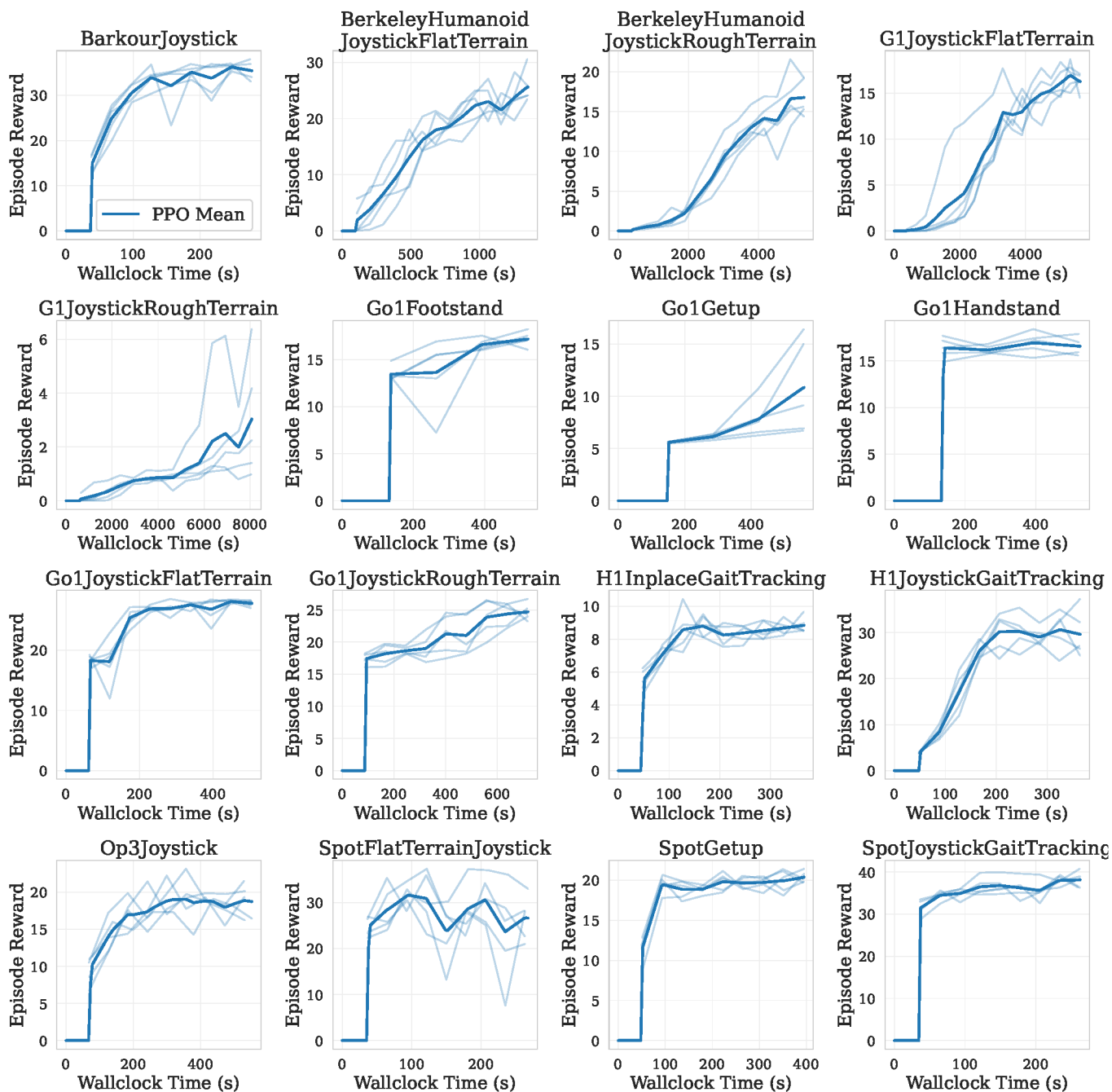
Fig. 12: Reward vs wallclock time for Brax PPO. All settings are run with 5 seeds on a single A100 GPU device. Notice that the initial flat region measures the compilation time for the training + environment code.
