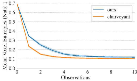
Fig. 13: Evaluation of the occlusion-aware information gain heuristic against a privileged clairvoyant view selection policy
