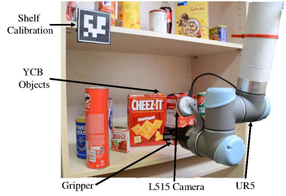
Fig. 4: Real-world environment showing a shelf scenario. The UR5 is equipped with a Robotiq parallel-jaw gripper and a Realsense L515 RGB-D camera to create a calibrated representation of the scene.
