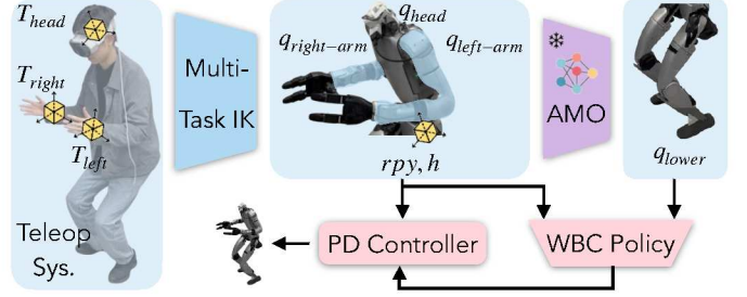
Fig. 3: Teleoperation system overview. The operator provides three end-effector targets: head, left wrist, and right wrist poses. A multi-target IK computes upper goals and intermediate goals by matching three weighted targets simultaneously. The intermediate goals (\mathbf{rpy}, h) are fed to AMO and converted to lower goals.
