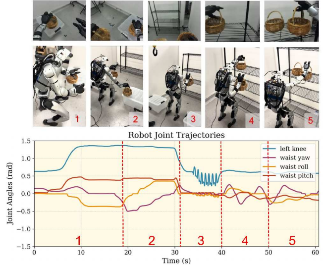
Fig. 7: Basket Picking: A complicated loco-manipulation task that also requires whole-body coordination. The task begins with the robot picking two baskets from left(1) and right(2), which are placed at low heights and close to the ground. Then, the robot stands up, moves forward(3), and puts two baskets on the shelf at eye level(4,5). The motor angle trajectories along the autonomous rollout are displayed and labeled to match the corresponding phases.
