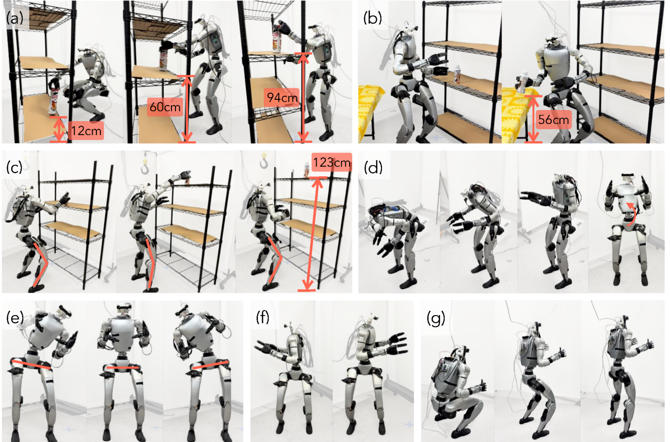
Fig. 1: AMO enables hyper-dexterous whole-body movements for humanoid robots. (a): The robot picks and places a can on platforms of different heights. (b): The robot picks a bottle from the higher shelf on the left and puts it on the lower table on the right. (c): The robot stretches its legs to put the bottle on a high shelf. (d-g): The robot demonstrates a wide range of torso pitch, roll, yaw, and height adjustments. (e): The robot utilizes hip motors to compensate waist joint limits to achieve larger roll rotation.
