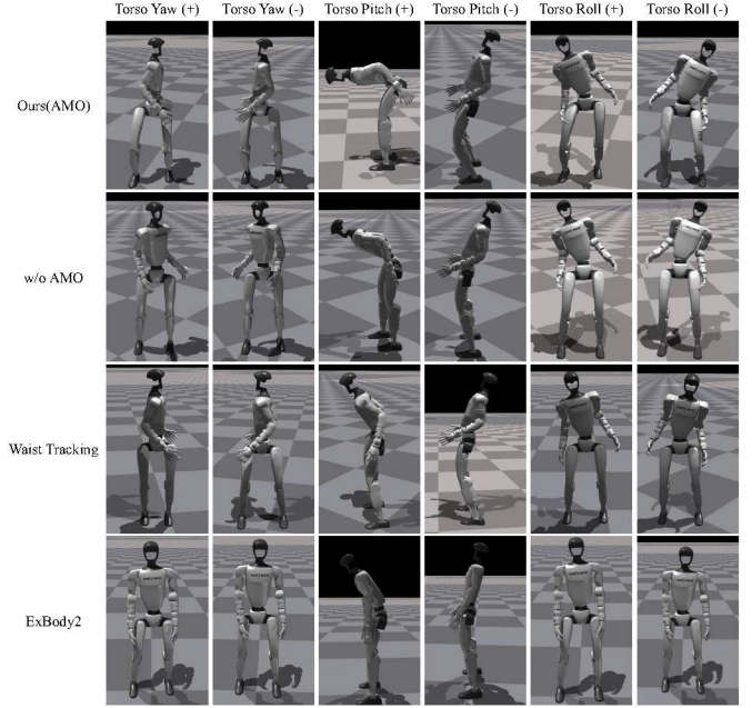
Fig. 4: Comparison of torso orientation ranges.
