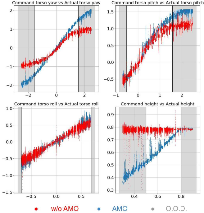
Fig. 5: Evaluation of in-distribution (I.D.) and out-of-distribution (O.O.D.) tracking results. Each figure shows the target vs. the actual commanded direction. The white area indicates I.D., meaning the command is used in both trajectory optimization and RL training. The grey area indicates O.O.D., meaning the command is not used in either trajectory optimization or RL training. The red and blue curves represent w/o. AMO and AMO , respectively.
