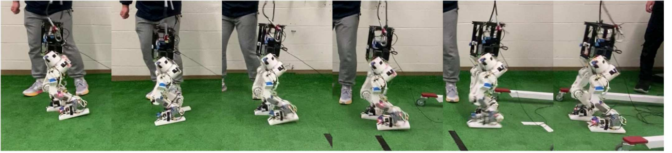
Fig. 14. Snapshot of the robot in bipedal configuration walking forward with a trained RL policy. The robot is able to track a user commanded velocity.
