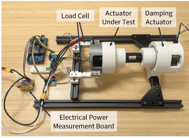
Fig. 7. Power efficiency test setup. Two load cells are used to directly measure the torque of the actuator under test, while another actuator acts as a damper, absorbing the mechanical energy produced by the actuator under test.
