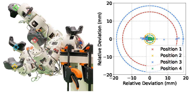
Fig. 12. (Left) The 5-DoF arm is commanded to reach four spatial position targets. (Right) End-effector position variance over 100 repetitions of the reaching task.
