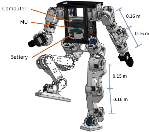
Fig. 2. Main components and key dimensions of the limbs of the Berkeley Humanoid Lite.
