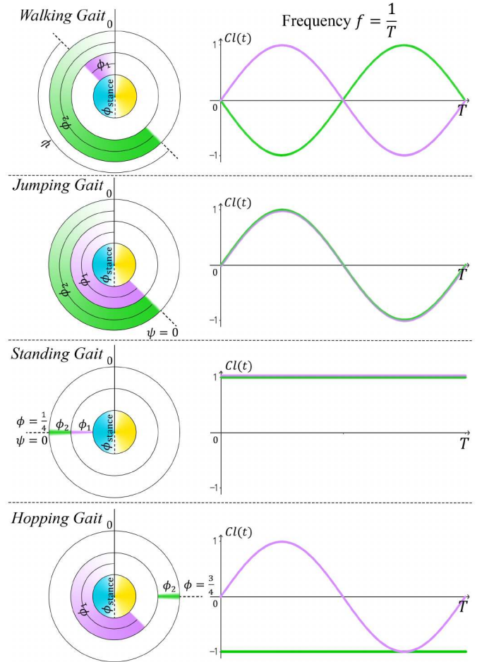
Fig. 4: Phase variables and clock functions under different gaits. Left: The purple ring represents the phase variable \phi_1 for the left foot, while the green ring represents the phase variable \phi_2 for the right foot. \psi is the phase offset from \phi_1 to \phi_2 . The dividing phase between stance (marked in blue) and swing (marked in yellow) is the duty cycle \phi_{\text{stance}}(0.5) . Right: The purple line depicts the clock function Cl_L(t) for the left foot over a cycle, while the green line represents the clock function Cl_R(t) for the right foot over a cycle.
