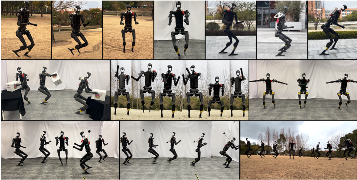
Fig. 1: Humanoid capabilities supported by HUGWBC. First row: HUGWBC allows four standard gaits - walking, jumping, standing, and hopping - with multiple customizable parameters to adjust the foot and pose behaviors, using one policy for 3 of the 4 gaits. Second row: HUGWBC supports real-time interventions from external upper-body controllers, enabling loco-manipulation while maintaining precise control under any locomotive behavior. Third row: Various command combinations enable the robot to perform highly dynamic movements.
