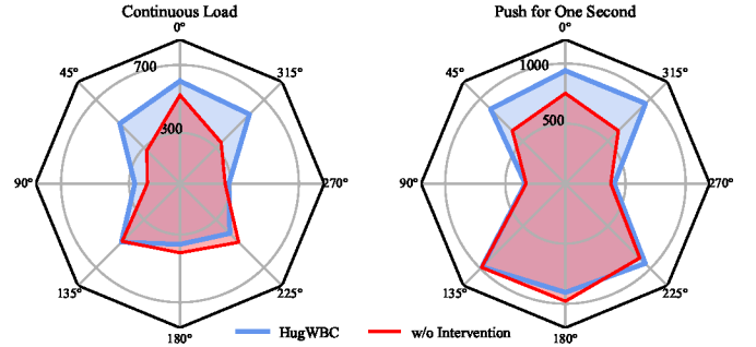
Fig. 6: External disturbance tolerance. Left: A constant and continuous force is applied to the robot. Right: A one-second force is exerted on the robot. The experiment is conducted under a standing gait with default commands. If the robot’s survival ratio exceeds 98%, it is deemed capable of tolerating such external disturbance. The survival ratio computes the trajectory ratio of non-termination (ends of timeout) during 4096 rollouts.
