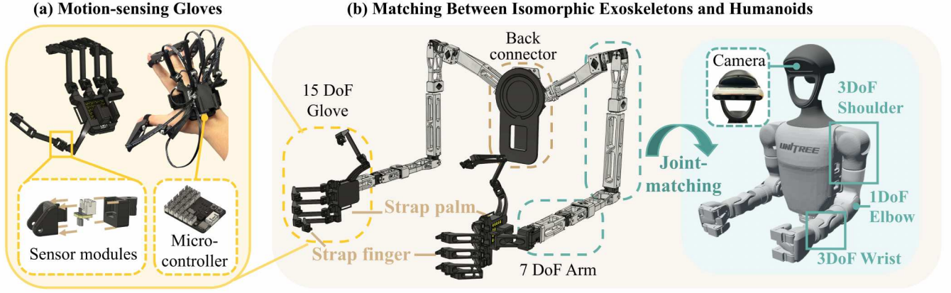
Fig. 5: Upper-body Exoskeleton. (a): The model architecture and physical demonstration of motion-sensing gloves. (b): The structural architecture of the upper-body exoskeleton system, comprising an isomorphic exoskeleton and motion-sensing gloves, with kinematic mapping methodology between the isomorphic exoskeleton and Unitree G1.
