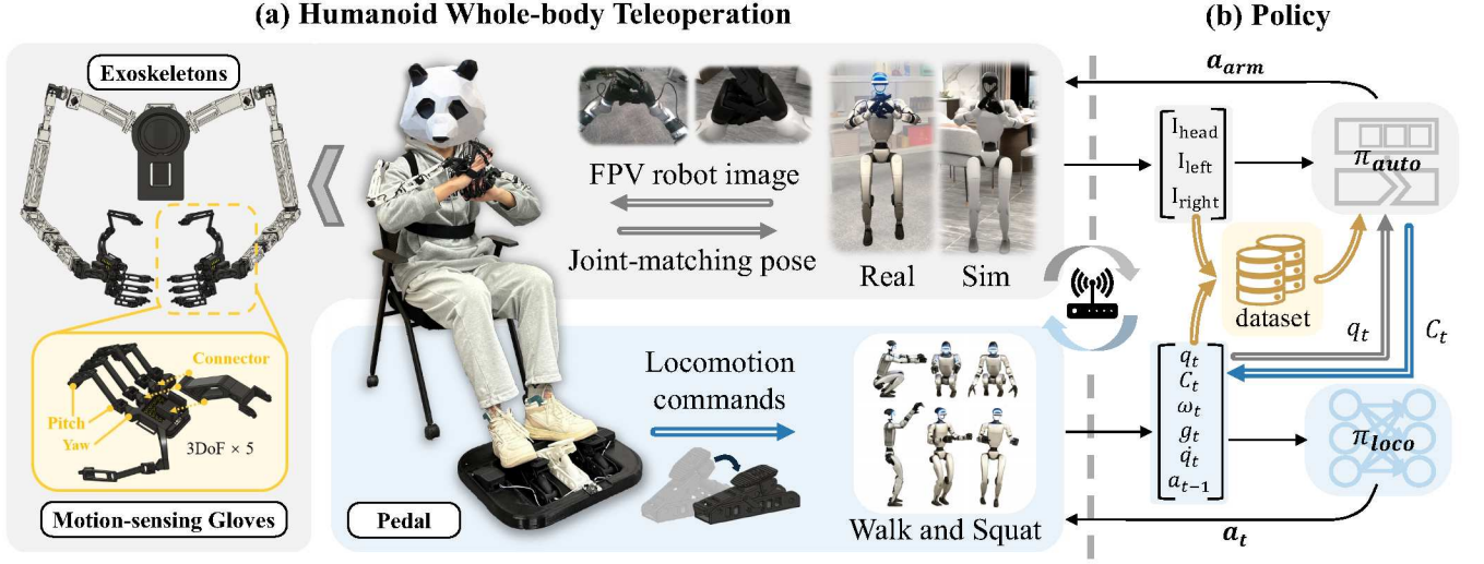
Fig. 2: System Overview. (a): how an operator uses the exoskeleton-based hardware system to control humanoid robots in the real world and simulation. (b): how \pi_{loco} controls the robots, the data collection process for training \pi_{auto} , and how \pi_{auto} takes over the operator to control the robots. Communication between the cockpit and the robot is achieved via Wi-Fi.
