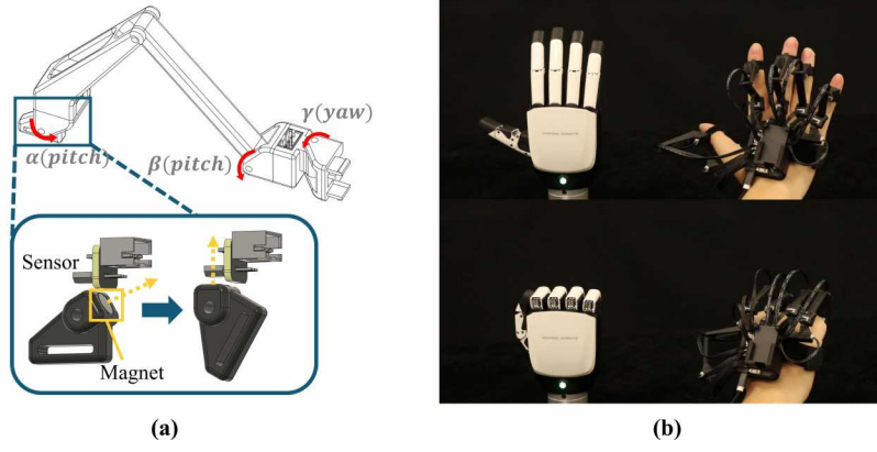
Fig. 20: (a): The schematic diagrams of the three degrees of freedom for each finger and the rotation of the magnet affecting the magnetic field direction. (b): Physical images of the Inspire Hands actual device in both open and clenched fist states.
