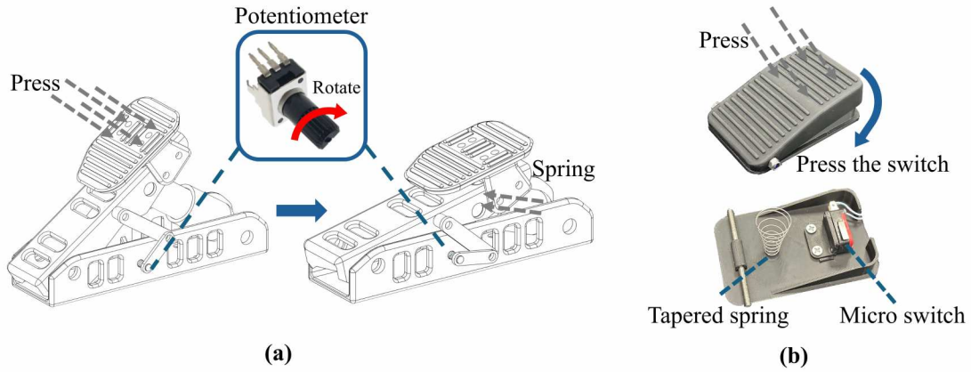
Fig. 21: (a): Schematic diagram of the small pedal principle, where the operator's foot press drives the potentiometer to rotate. (b): Schematic diagram of the mode-switching buttons, where the operator's foot press changes the state of the micro switch.
