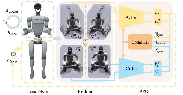
Fig. 3: RL training framework of HOMIE.
