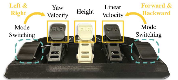
Fig. 6: Pedal command control. The three small pedals respectively control [0, \pm\omega_{max}] , [H_{min}, H_{max}] , and [0, \pm V_{max}] . The left-side switching button is used to toggle between left and right modes, while the right-side switching button is used to toggle between forward and backward modes.
