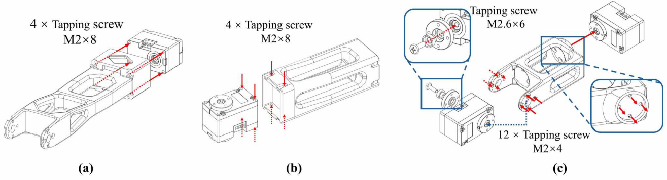
Fig. 18: The assembly methods of the servos and structural components, along with the screw requirements, are as follows: (a), (b:) The structural components are directly assembled and fixed to the servo body; (c:) The structural components are assembled and fixed to the servos via one or two servo disks, respectively.
