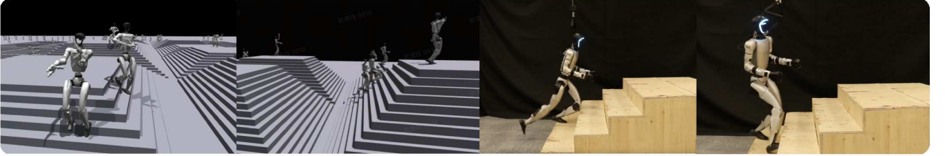
Fig. 17: Training robots to traverse stairs. Left: Training in simulation; Right: Deployment in the real world.
