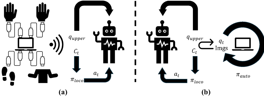
Fig. 22: Deployment of our system with cockpit and autonomous policy. (a): Deployment with robot controlled by isomorphic exoskeleton cockpit. (b): Deployment with robot controlled by autonomous policy \pi_{auto} .
