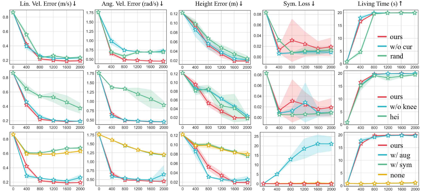
Fig. 7: Ablation experiments of our RL training framework. Each row from top to bottom represents the ablation study for upper-body curriculum, height tracking reward, and symmetry utilization, respectively. Each column represents the evaluation of the corresponding metrics for checkpoints under different ablation settings. The \uparrow and \downarrow symbols beside the metrics indicate whether a higher or lower value is better for the respective metric.
