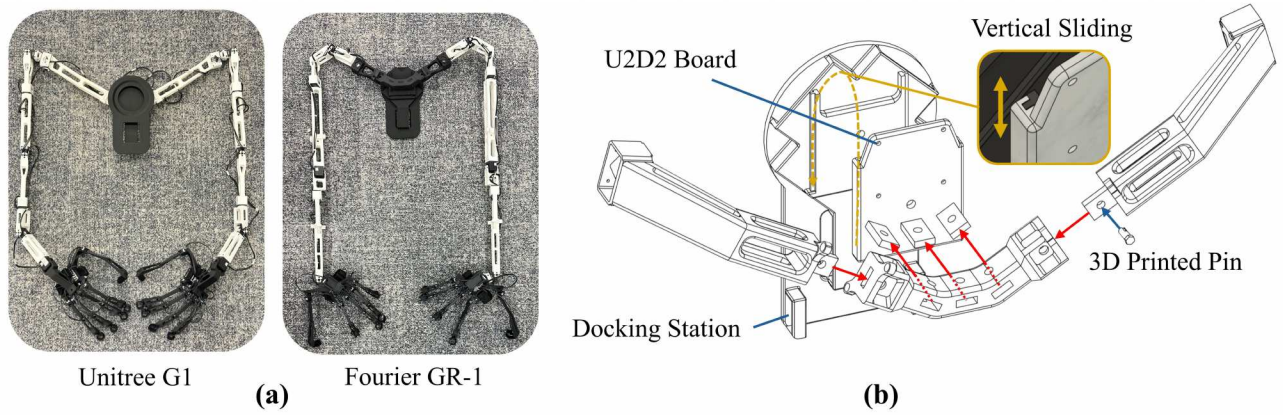
Fig. 19: (a:) Physical models of two different Humanoids' Isomorphic Exoskeletons, equipped with servos, back connectors, and motion-sensing gloves; (b:) Schematic diagram of the back connector assembly and functionality, where the connectors can be fixed using a dovetail structure and plugs. The U2D2 board and docking station are external physical components.
