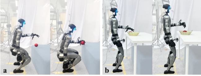
Fig. 15: Autonomous policy controlling robot to perform tasks. a: Squat Pick; b: Pick & Place.
