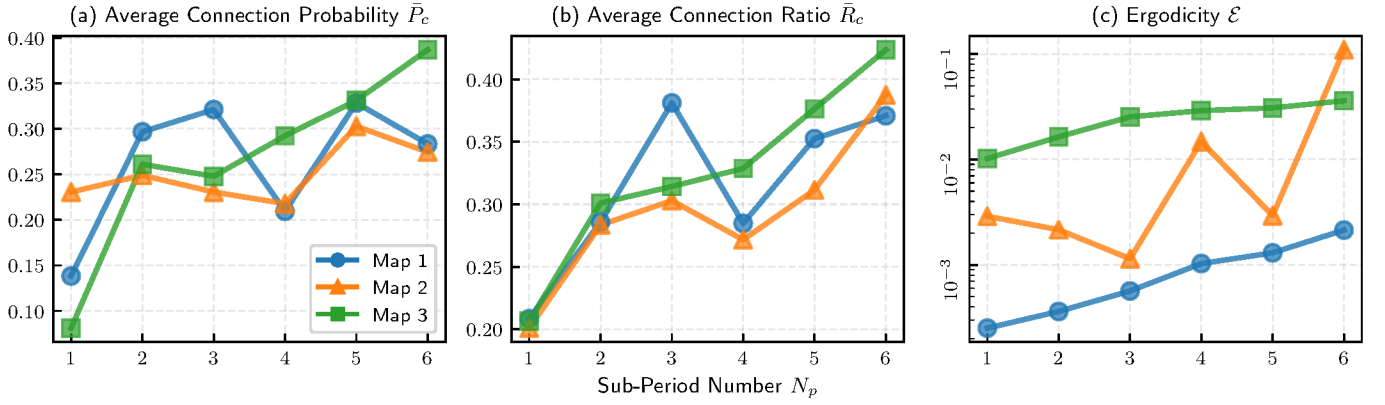
Fig. 4. Illustration of the impact of varying sub-period numbers on the following performance indicators (a): average connection probability \bar{P}_c , (b): average connection ratio \bar{R}_c , (c): ergodicity \mathcal{E} .
