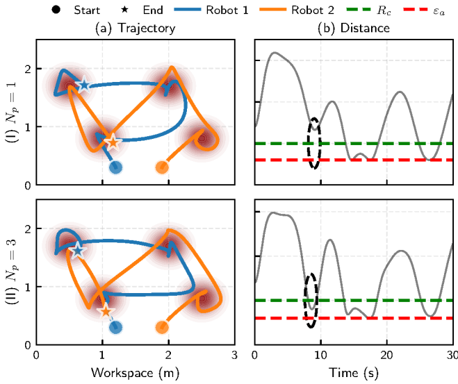
Fig. 5. Comparison of robot trajectories and inter-robot distances for sub-period numbers N_p \in \{1, 3\} . (a): Robot trajectories, (b): Inter-robot distance over time, where R_c and \epsilon_a denote the connection range and the collision avoidance threshold.
