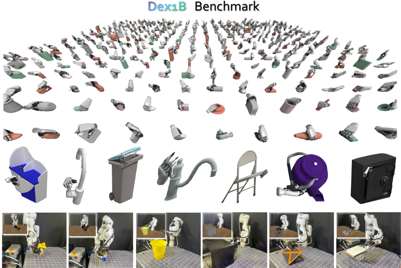
Fig. 1: The Dex1B benchmark consists of 1B generated high-quality demonstrations for grasping and articulation tasks. In the bottom row, we show the deployment results of the simulation (small image) and real world (big image) using DexSimple trained with Dex1B. This demonstrates that Dex1B is scalable and generalizable to real environments.
