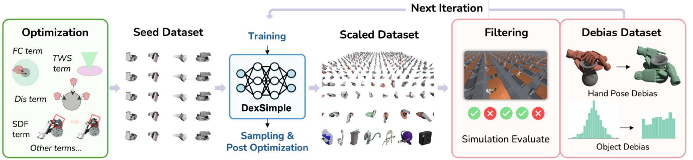
Fig. 2: DexIB demonstration collection. The engine takes object assets and hand pose initialization as input, using a control-based optimization algorithm to generate the Seed dataset. Then the Seed dataset is used as the training data for DexSimple, else for Dex1Bfor the last iteration. Then DexSimple will generate a scaled proposal dataset with \pi as the scaling ratio. For the proposal dataset, we then use the simulation critic and debiased algorithm to create the debiased dataset for optimization refinement.
