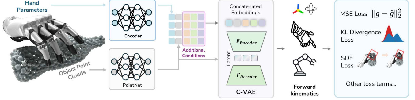
Fig. 3: DexSimple Pipeline. Our model takes in hand parameters and object point clouds as fixed input for CVAE, while root rotation, translation, and joint value as optional conditions. Those are combined as the input embeddings for CVAE, while point cloud embeddings are re-emphasized at the latent space. The output of CVAE is the forward kinematics define the hand pose trajectory optimized by the effective loss function.
