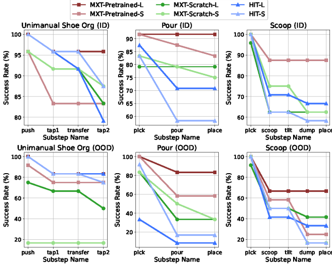
Fig. 6: Substep success rate. The success rate for some substep is calculated as the percentage of trials where the robot successfully completed the substep. For each task, we calculate this with 24 ID rollouts and 12 OOD rollouts. MXT-Pretrained : MXT pretrained on human dataset (including unimanual and bimanual if applicable), then finetuned on the LocoMan data. MXT-Scratch : MXT trained only on the LocoMan data. “L” denotes the larger training set (80 trajectories for SO-Uni, 60 trajectories for Pour and Scoop), while “S” denotes the smaller training set (40 trajectories for SO-Uni, 30 trajectories for Pour and Scoop).
