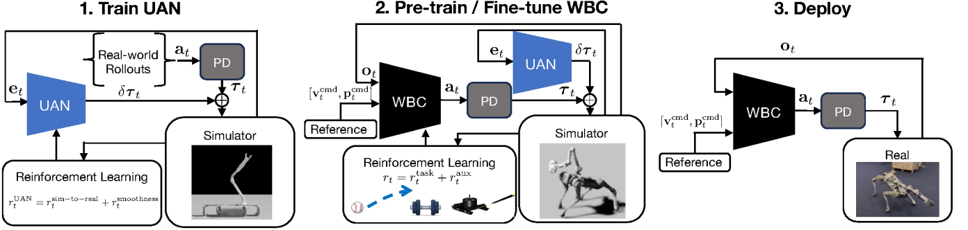
Fig. 2: Unsupervised Actuator Network (UAN) approach for real-to-sim-to-real. Our training pipeline involves three steps: 1) Train a UAN to close the sim-to-real gap for actuators with complex transmission mechanisms by mapping a history of joint position and velocity errors, \mathbf{e}_t , to corrective torques, \delta\boldsymbol{\tau}_t , 2) Pre-train a WBC using random motion references (base velocity and EE pose), then and fine-tune it on an athletic task reward with the UAN in loop, and 3) Deploy. During the fine-tuning phase, the WBC initially tracks the task-specific reference, and then gradually learns to depart from the reference to maximize task performance.
