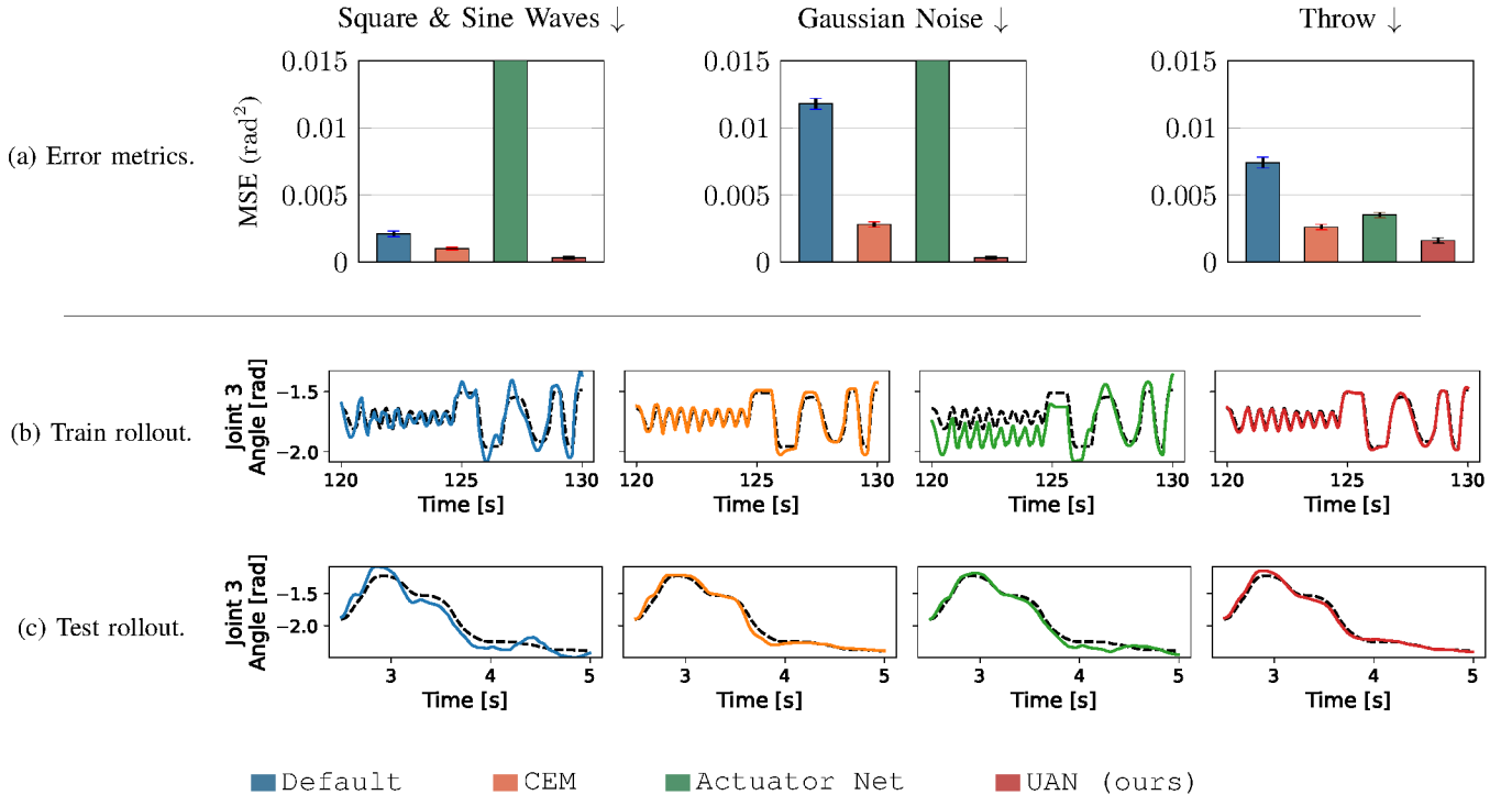
Fig. 6: UAN achieves the tightest real-to-sim fit to the training data, as well as a throw trajectory unseen during training. We rolled out three real-world joint trajectories: square & sine waves at each joint, Gaussian noise across all the joints, and a throw. Square waves, sine waves, and gaussian noise were seen during training, while the throw was not. We found that Actuator-Net error remains bounded on the 5s throw trajectory but diverges when rolling out the 5 min training trajectories, while the UAN learned to remain accurate across long rollouts through RL training. The dashed lines in (b) and (c) are the positions realized on hardware.
