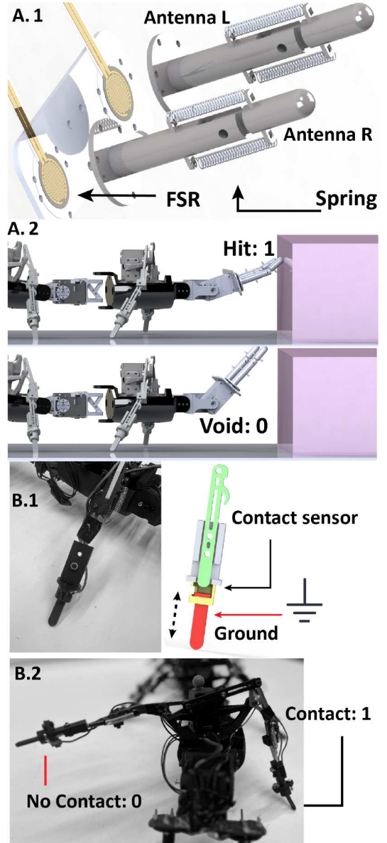
Fig. 3. Tactile sensory system. A. Antenna design. A1. The base of the antenna is attached to a Force Resistive Sensor (FSR) using screws. The inner part of the antenna is connected to its tip with two springs, allowing it to deform upon contact with obstacles, thereby preventing jamming. A2. Antenna contact states: A value of 0 represents no contact (void state), while 1 indicates an obstacle has been detected. B. Binary limb contact sensing system. B1. Design of a binary contact sensor for each foot, based on capacitive sensing. B2. Contact state of the leg: 0 indicates no contact, while 1 indicates contact.
