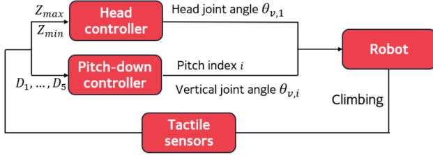
Fig. 7. Feedback control framework for climbing. Two parallel controllers independently manage the pitch motion of the head segment and a subsequent segment. Using the Z -positions ( Z_{max} and Z_{min} ) of the obstacle measured by the antenna, the head controller adjusts the head segment to closely follow the contour of the obstacle. Based on the duty factors ( D_1, \dots, D_5 ) measured by foot contact sensors, the pitch-down controller identifies the appropriate floating segment nearest to the edge and pitches it down to accelerate the transition from floating to being positioned on top of the obstacle.
