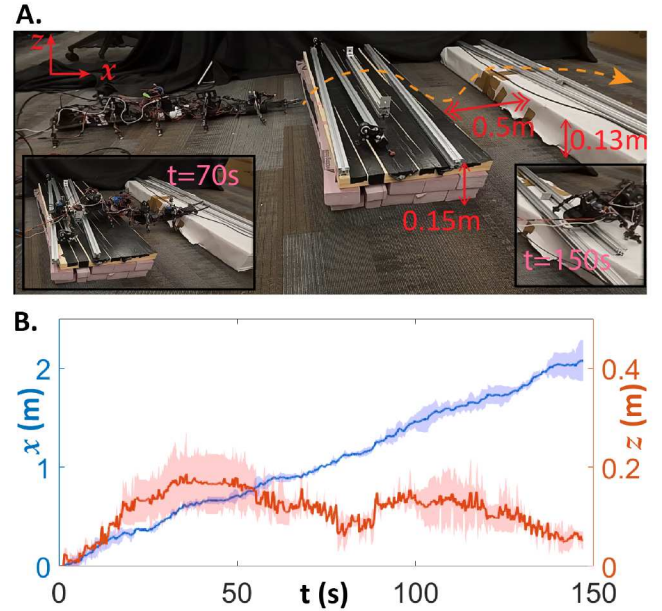
Fig. 11. Traversal of two consecutive obstacles A. Snapshots showing the robot traversing two obstacles (0.15 m and 0.13 m in height, spaced 0.5 m apart) within 150 s. B. Forward ( x ) and vertical ( z ) displacement across five trials. Shaded regions represent the standard deviation.
