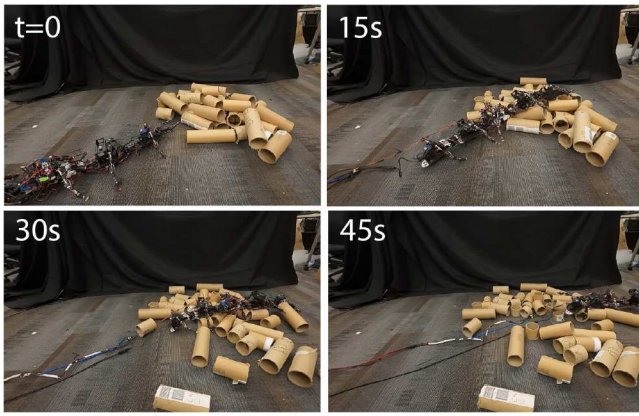
Fig. 12. Robot navigating unstable obstacles. Snapshots show the robot traversing a pile of unstable, shifting obstacles — 9 cm diameter cylinders of varying lengths (5 – 15 cm), covering a 60 cm × 60 cm area and reaching up to 20 cm in height.
