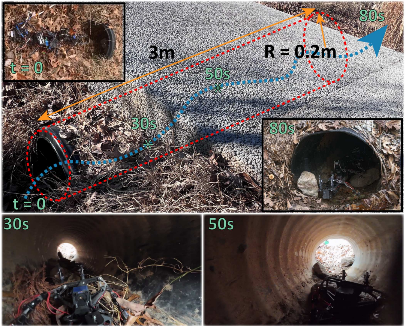
Fig. 13. Robot traverses a pipe. The robot completed an “inspection” task in 80 seconds within a cylindrical pipe measuring 0.2 m in radius and 3 m in length. The pipe contained randomly placed robot-sized rocks, requiring the robot’s climbing capability, while leaves and pine straw introduced entanglement challenges, increasing task complexity. A camera mounted on the robot captured footage during the traversal.
