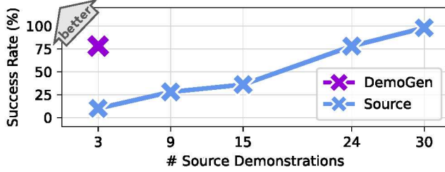
Fig. 21: Real-world comparison between DemoGen -generated and human-collected datasets. The DemoGen -generated dataset is based on 3 source demonstrations.
