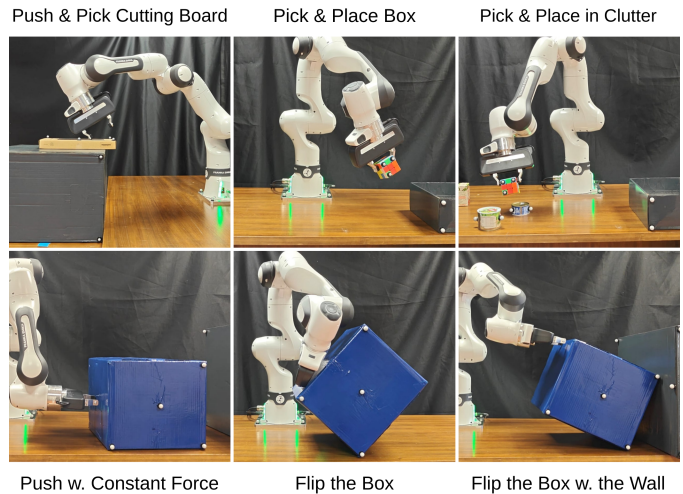
Fig. 1: Real-world execution of CoRAL across six different manipulation tasks.
