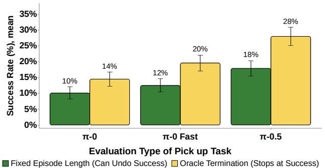
Fig. 18: Comparison of oracle termination and fixed-horizon termination for the pick task using \pi policies.
