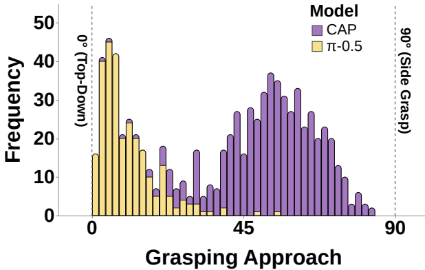
Fig. 9: Grasp direction histogram of successful grasp of the \pi_{0.5} and CAP policies. These policies are heavily biased towards top-down and side grasps respectively. The robots are also initialized in different configurations.
