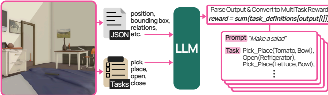
Fig. 4: The LLM-based long-horizon task generation system makes use of text-form scene descriptions to generate new task descriptions and success condition checks based on predefined atomic checks.
