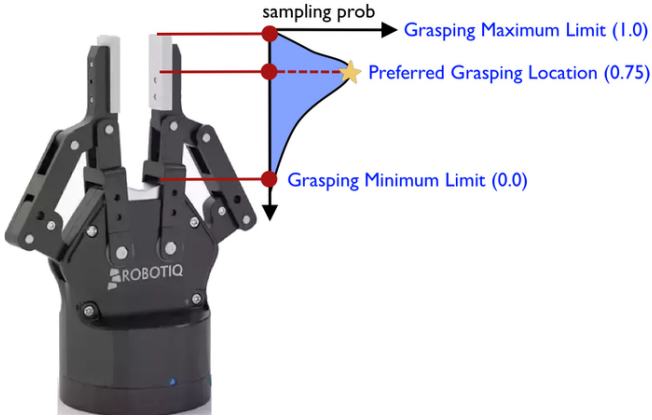
Fig. 17: RobotIQ 2F-85 gripper and preferred grasping locations for sampling grasps
