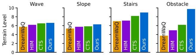
Fig. 5: Comparison of maximum terrain levels across varying friction coefficients as evaluated by RoboGauge.
