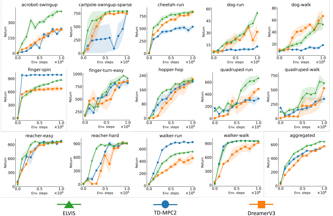
Fig. 4: DMC visual control learning curves. Per-task learning curves on 14 DeepMind Control (DMC) visual control benchmarks, together with an aggregated score that reports the mean episodic return averaged across all 14 tasks at each environment step. Shaded regions denote 95% confidence intervals over 5 random seeds. ELVIS achieves the strongest overall performance, ranking first or second on every task.
