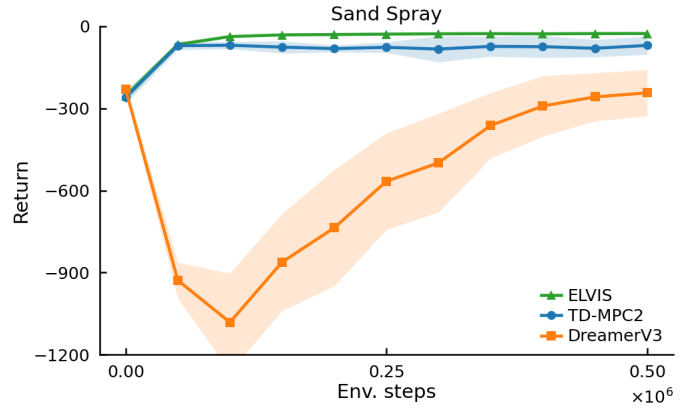
Fig. 7: Learning curves of simulated sand spray task. Scores of ELVIS, TD-MPC2, and DreamerV3 on the simulated sand spray task, which shows the mean episodic return at each environment step. Shaded regions denote 95% confidence intervals across 5 seeds. ELVIS significantly outperforms DreamerV3 while exhibiting more stable learning and reduced sensitivity to random seeds compared to TD-MPC2.
