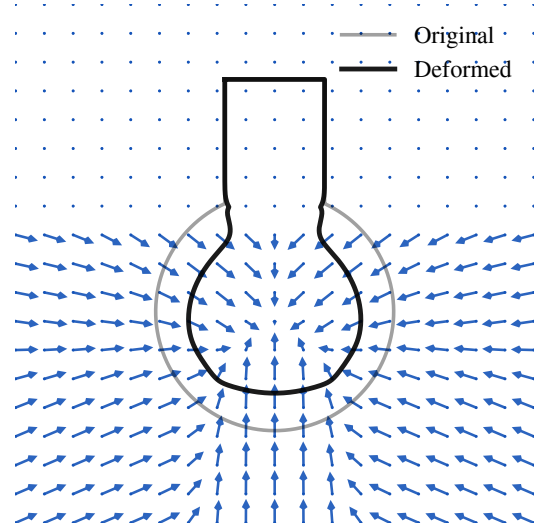
Fig. 3. Deformation of a 2D gripper contour under a stationary velocity field (SVF). The upper region is frozen (zero velocity), while the lower region deforms smoothly.
