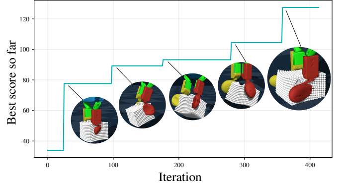
Fig. 5. End-effector design evolution for grasping a large jelly cube during a typical optimization run. High-scoring designs exhibit larger contact surfaces, which improve grasp stability and reduce contact-induced stress.
