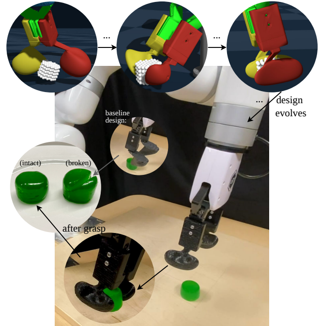
Fig. 1. We jointly optimize end-effector morphology and motion-adaptive control to enable safe, gentle manipulation of deformable and fragile objects. The co-designed end-effector reshapes contact geometry and force distribution, achieving reliable grasping while preserving object integrity, where baseline designs fail and cause breakage.
